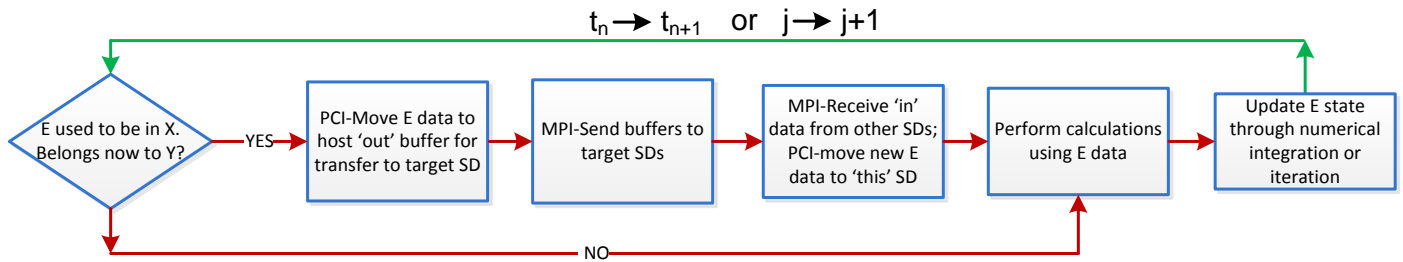
Figure 3: DDEP control flow. E stands for “element”, SD stands for “sub-domain”. Diagram captures what happens when advancing simulation to the next time step t_n \rightarrow t_{n+1} or moving from iteration j to j + 1 .
