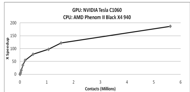
Figure 11: Overall speedup when comparing the CPU algorithm to the GPU algorithm. The maximum speedup achieved was approximately 180 times.
